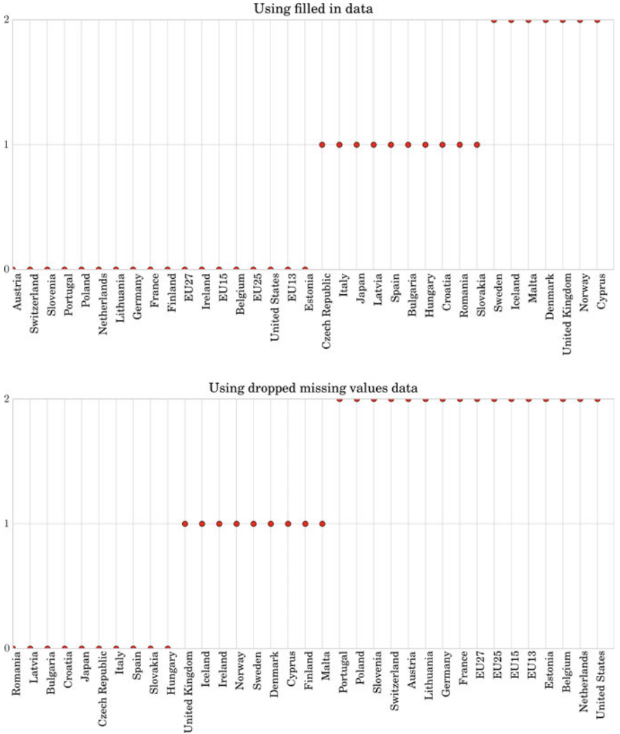
Fig. 7.9 Clustering of the countries according to their educational expenditure using filled-in ( top row ) and dropped ( bottom row ) missing values
