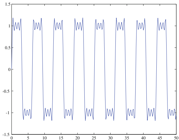
Fig. 2.2 A periodic signal approximated by 4 Fourier components
