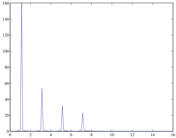
Fig. 2.3 Frequency spectrum
