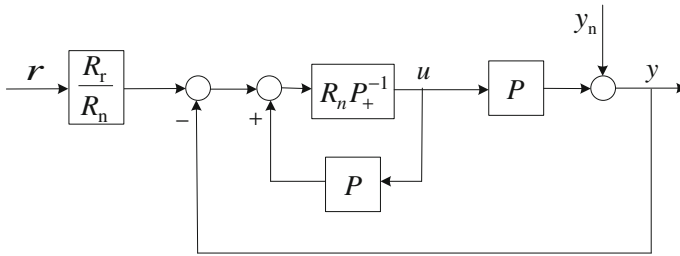
Fig. 7.9 Equivalent control scheme
