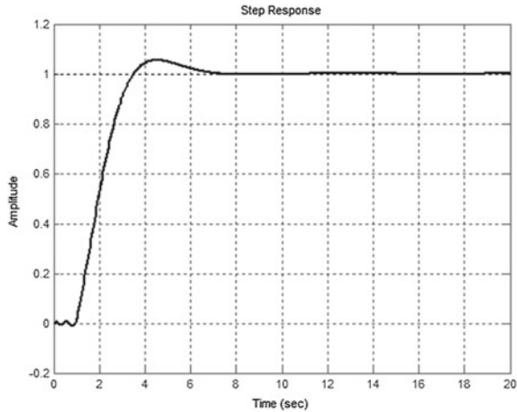
Fig. 8.13 Step response of the control system
