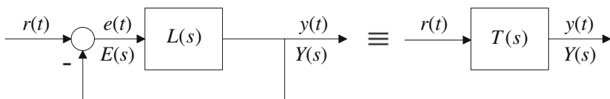
Fig. 4.1 Negative feedback
