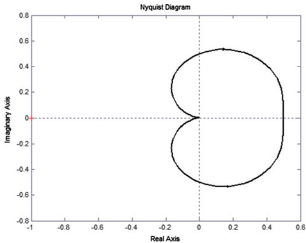
Fig. 1.5 NYQUIST diagram
