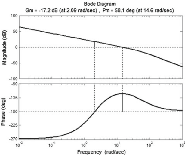
Fig. 8.19 BODE diagram of PID control of an unstable process with phase margin of 60^\circ
