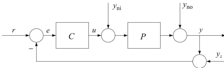
Fig. 7.1 Block diagram of a control system
