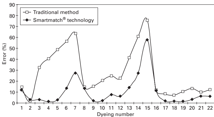
2.8 Graphical representation of the concentration deviation for a quadrichromy.
