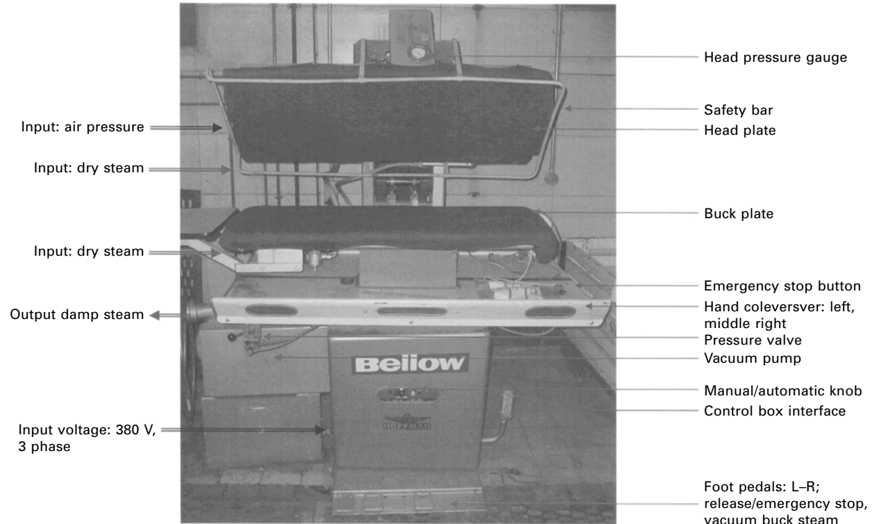
12.3 The Hoffmann steam press.
