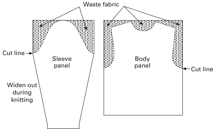
9.2 Knit to width and widen.
