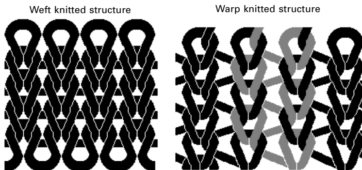
9.1 Knitting construction methods.
