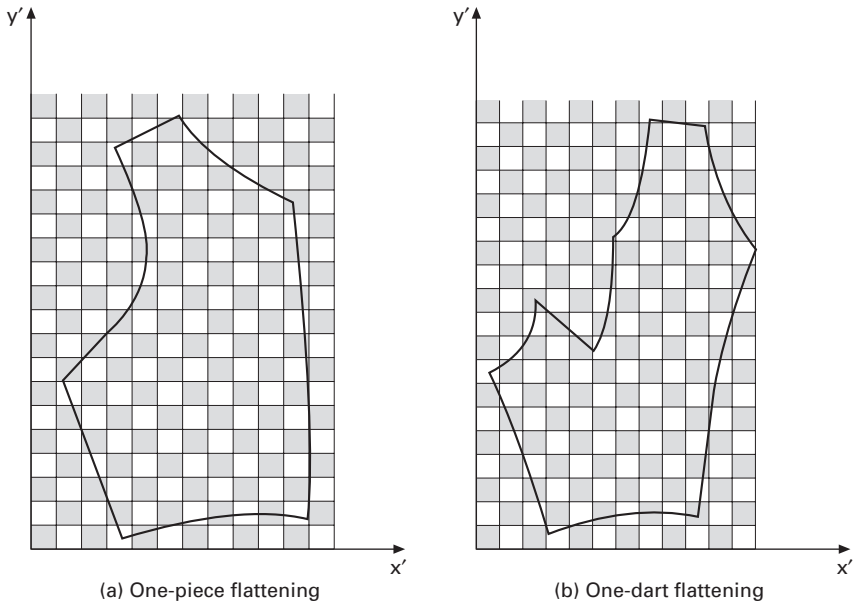
6.9 Two-dimensional pattern overlay on fabric texture.
