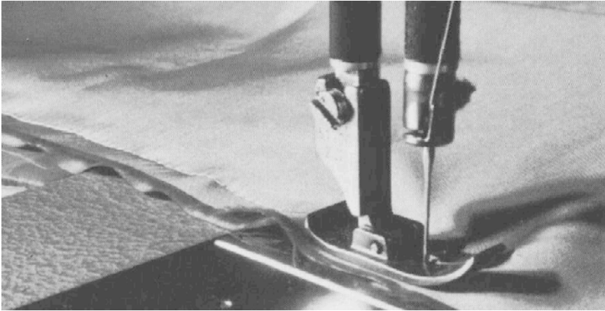
13.2 Example of feed pucker.
