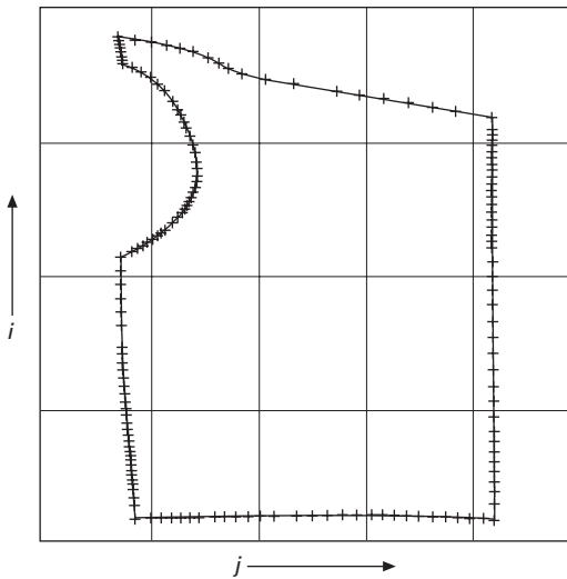
(b) Intensification of panel boundary nodes
