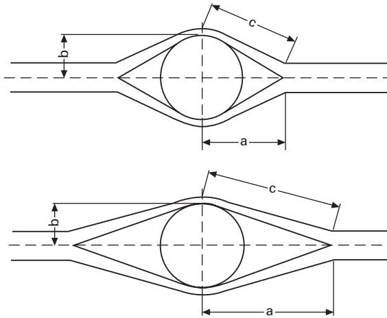
13.1 Structural jamming of the sewing thread between the yarns in the fabric. 7
