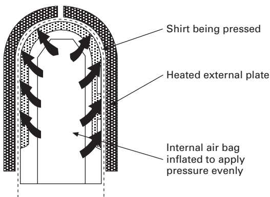
12.7 The Veit TwinStar shirt press utilises heated external shaping plates in conjunction with an internal air bag which inflates to apply even pressure to the garment. (Courtesy of Veit GmbH, Landsberg/Lech, Germany.)
