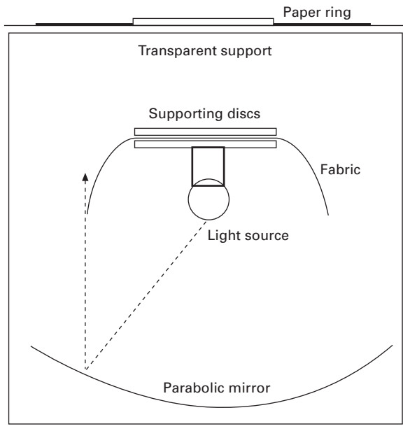
1.1 Cusick's drapemeter. Source: Chung. 11
