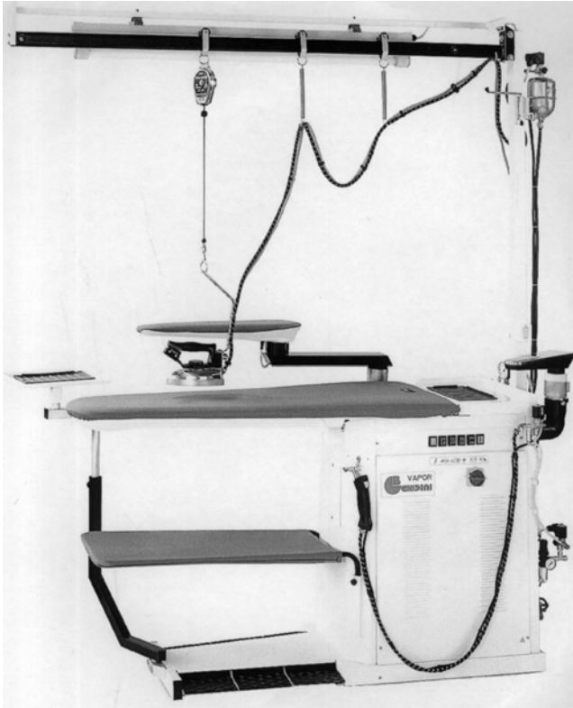
12.2 Dress board ironing station with both air suction and blowing. The unit is shown with a swivel arm and sleeve buck; it also has a cantilever iron support gantry. (Courtesy of Ghidini Benvenuto SRL, Milan, Italy.)
