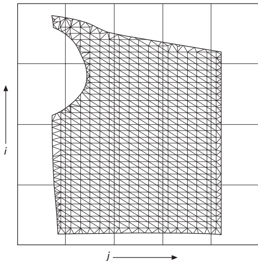
(d) Triangulation of panel boundary and interior nodes
