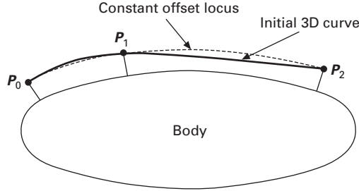
(b) Initial 3D curve through points
