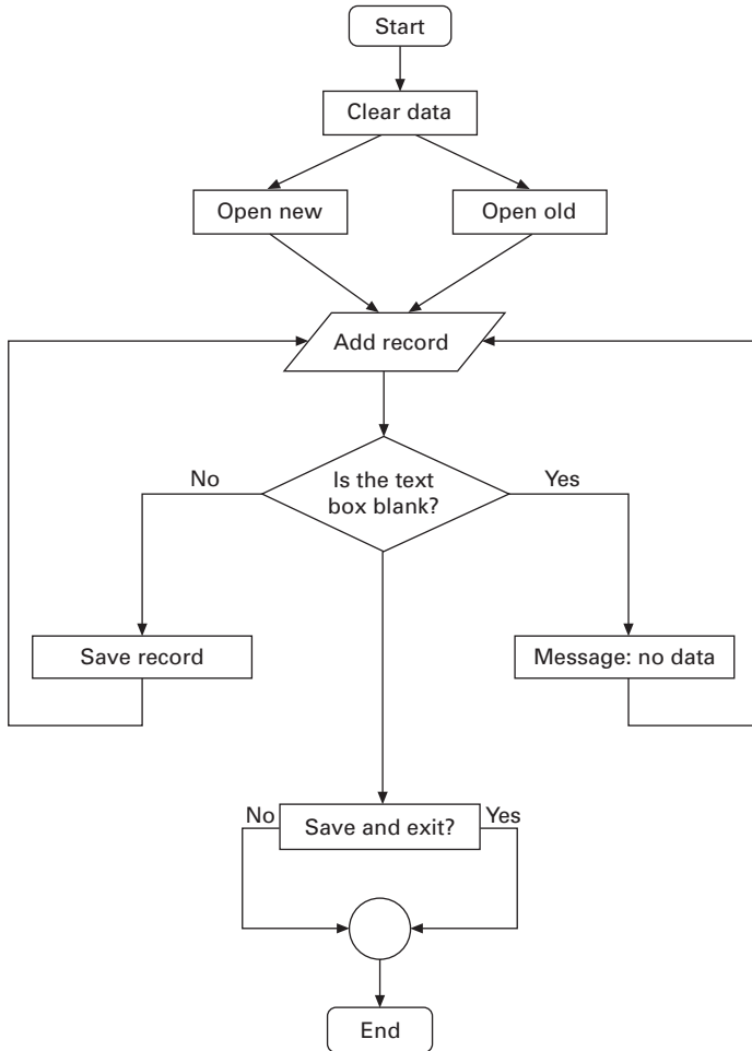
13.17 Database algorithm.
