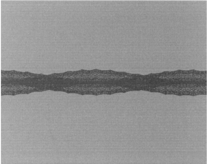
3.2 Mesh surface.
