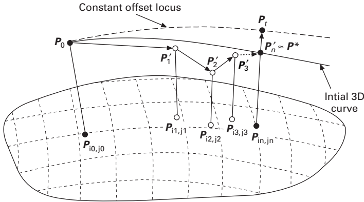
6.3 Constant offset compilation using Newton–Raphson search.
