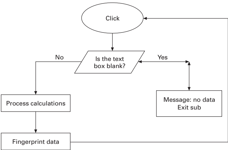
13.19 Fingerprint algorithm.
