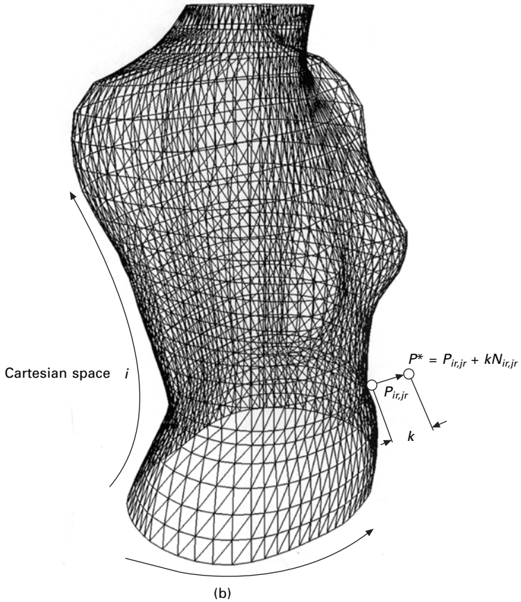
6.1 Mapping of parametric space coordinates to Cartesian space.
