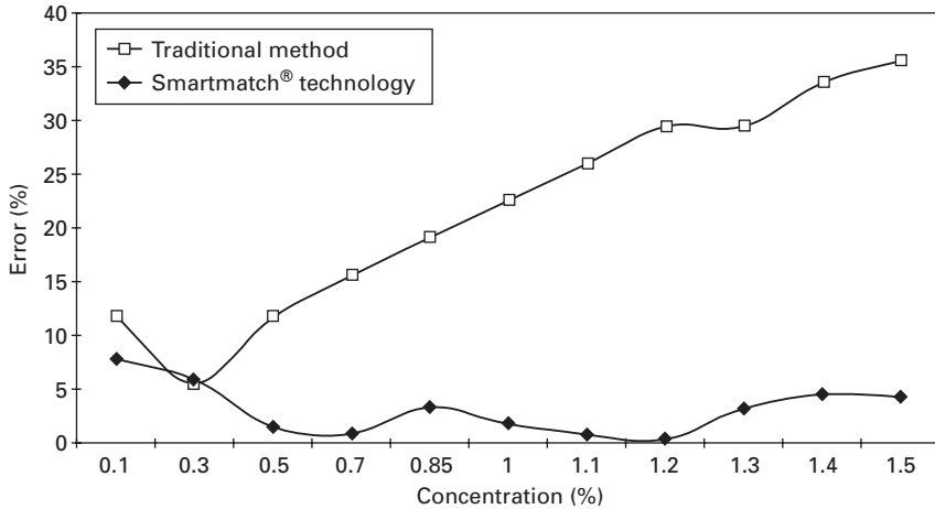
2.6 Graphical representation of the concentration deviation for a trichromy.
