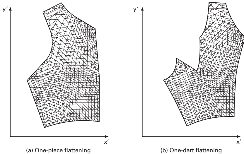
6.8 Initial 2D pattern triangulation.
