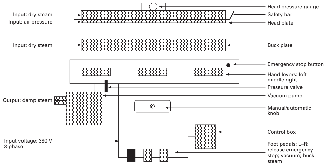
12.4 Schematic diagram of the Hoffmann steam press.
