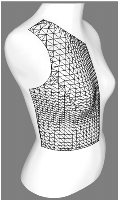
(a) Panel triangulation
