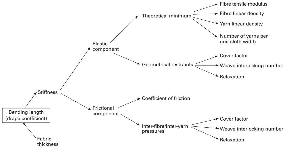
1.3 Some factors contributing to fabric drape behaviour. Direction of arrows indicates whether an increase or decrease in a given parameter will produce an increase in the drape coefficient of the fabric. Source: 18,19
