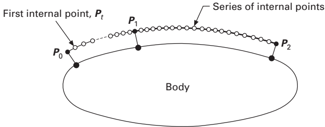
(c) Final piecewise interpolated 3D curve at constant offset kr
