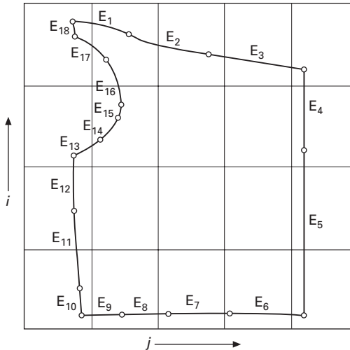
(a) Initial design point and curve specification of panel
