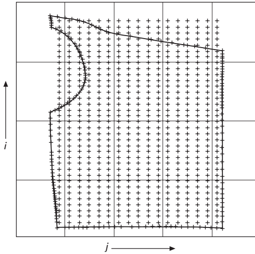
(c) Floodfill with panel interior nodes
