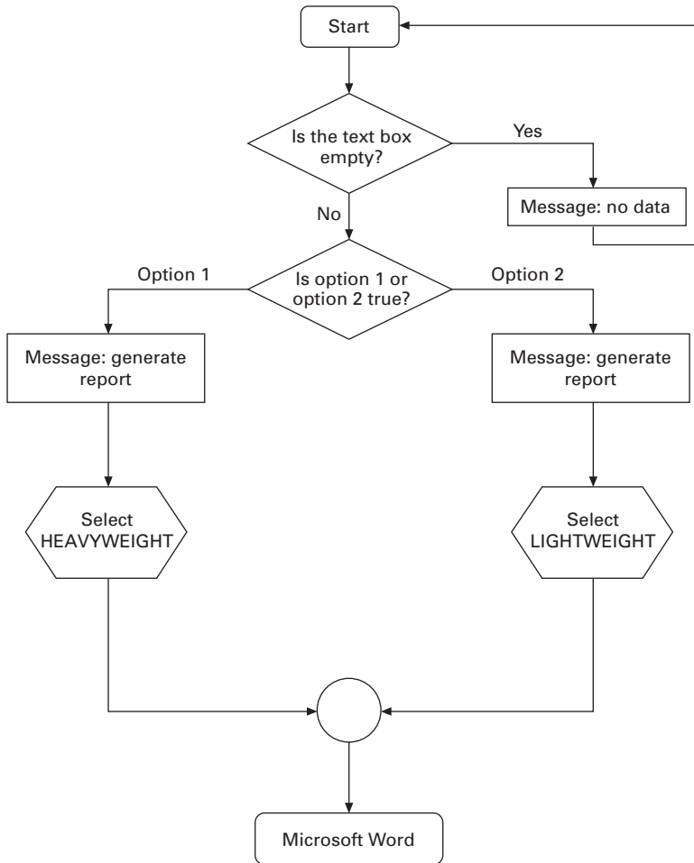
13.20 Report generation algorithm.
